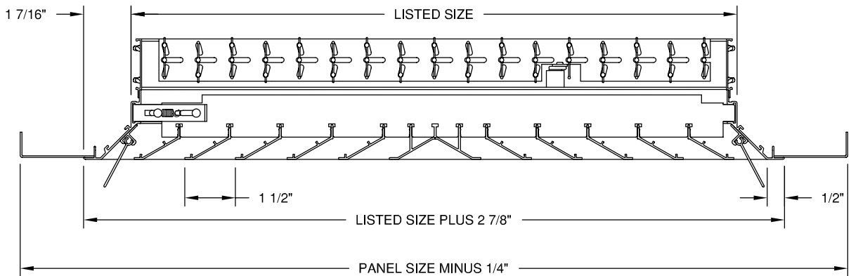
MODEL - AMD-T-ALIP - SHOWN WITH OPTIONAL DEFLECTOR AND OPPOSED BLADE DAMPER
